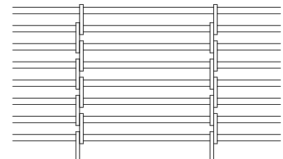
'HL9' Heavy Link 3/16" 2-Hole Links Links 9" OC - Rods 1 1/2" OC (Models PG, HG*)
