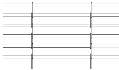
'CL9' Compact Link 1/8" 2-Hole Links Links 9" OC - Rods 2" OC (Models CG, SG*, HG*)
