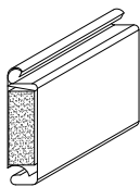
Type 'Ti' Insulated Slat EPS Foam / PVC Back 2 5/8" x 13/16" (Models MI, HI*)
