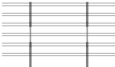
'SL9' Straight Link Alternating 1/8" & Double 1/16" 3-Hole Links Links 9" OC - Rods 2" OC (Models SG, HG)
